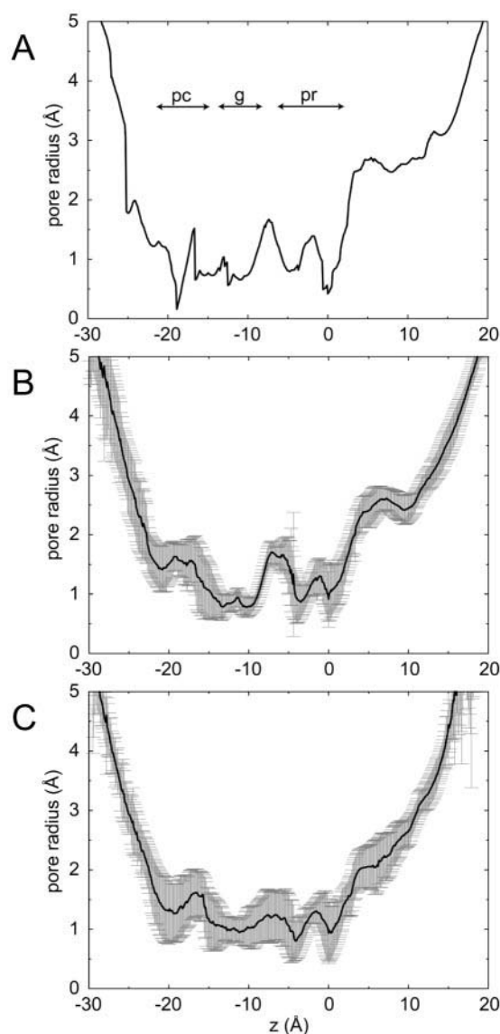
FIGURE 8 Pore radius profiles (produced using HOLE (Smart et al., 1996)). (A) The pore profile for the starting model of OmpA 171 is shown, and the major constrictions (pc, periplasmic cover; g, gate; pr, polar ring) to permeation are indicated. (B) The trajectory-averaged pore profile with standard deviation bars (gray) for the most stable octane simulation, Med_Oct, reveals that only around the Arg138-Glu52 gate region is the pore radius unlikely to expand to the minimum dimensions required for a water molecule to pass. (C) The trajectory-average pore profile with standard deviation bars for the simulation of the modeled OmpA 171 open state is shown. Notice that now the pore radius around the gate region is able to expand beyond 1.15 Å.
