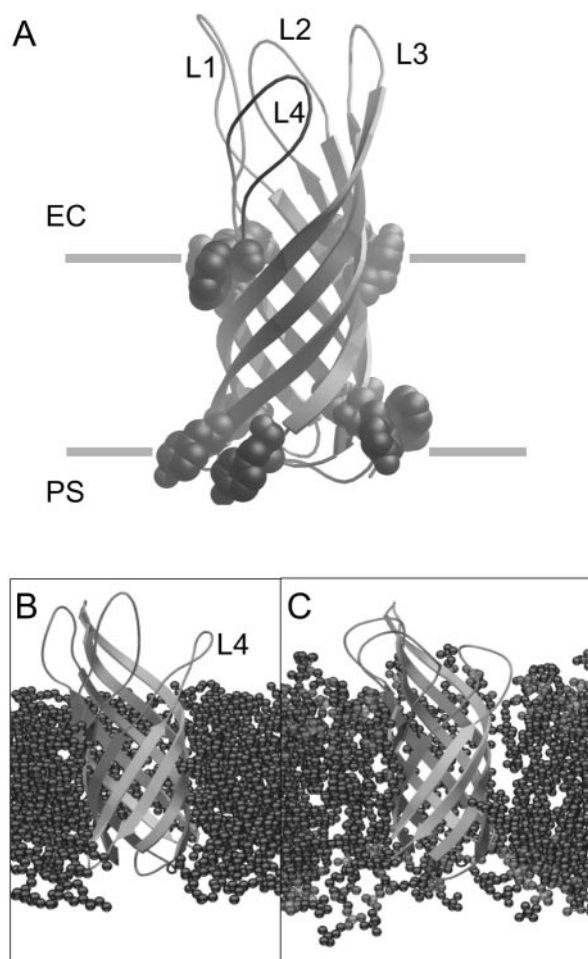
FIGURE 1 ( A ) Schematic diagram of the OmpA N-terminal domain (drawn using VMD (Humphrey et al., 1996, and Povray ( http://www.povray.org )) showing the two bands of amphipathic aromatic side chains (i.e., Trp and Tyr) and the presumed location of the membrane (horizontal gray lines). The extracellular loops (L1 to L4) are labeled. ( B and C ) Snapshots of simulation systems: Med_Oct ( B ) and DMPC ( C ) (drawn using Molscript (Kraulis, 1991) and Povray), showing the protein (in ribbons format colored from blue (N-terminus) to red (C-terminus)) and the octane slab (black) or DMPC bilayer (fatty acid tails in black; PC headgroups in red/blue/pink). Water is not shown for clarity. The L4 loop is labeled.
