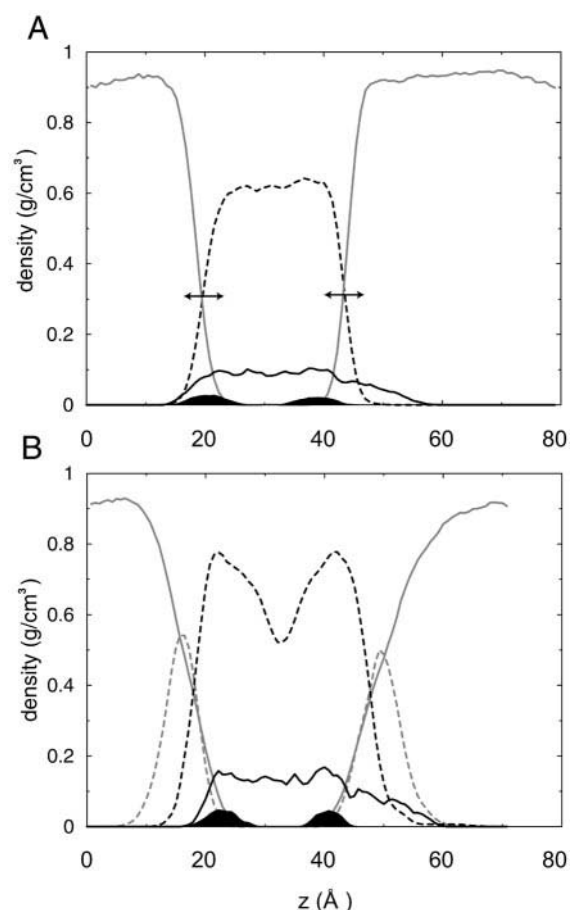
FIGURE 4 Trajectory-averaged system density as a function of the z coordinate for Med_Oct ( A ) (with arrows representing variation in width of octane slab density for Small_Oct and Big_Oct) and the DMPC simulation ( B ). The protein aromatic belts (black filled areas) can be seen to localize at the interface between the octane ( A ) (black dashed line)/water (solid gray line) interface, or the lipid tail ( B ) (black dashed line)/polar headgroup (gray dashed line) and water (solid gray line) interface. The lower aromatic belt (at z \approx 25 Å) localizes better with the polar/hydrophobic interfaces in each case, whereas the overall protein density (solid black line) is preferentially shifted toward the extracellular side.
